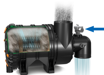
Impulse Cleaning with pressurized air if a certain dust loading condition is reached (e.g. time or pressure rise based)
