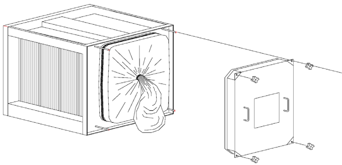
Fig. 6: Note bag safety strap and cinch strap)
