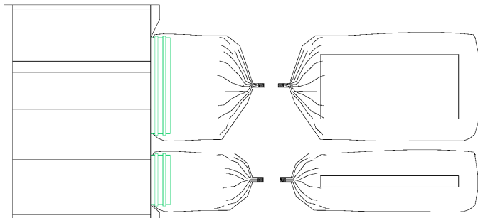
Fig. 13: Top view of both a prefilter and HEPA filter change out sealing lip in green
