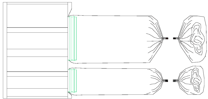
Fig. 11: Residual filter bag stubs of both prefilter and HEPA filter
