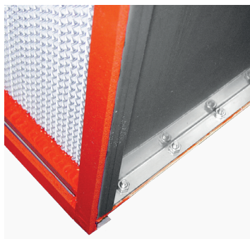
Close-up of Microbarrier HEPA HT frame media pack & sealant
